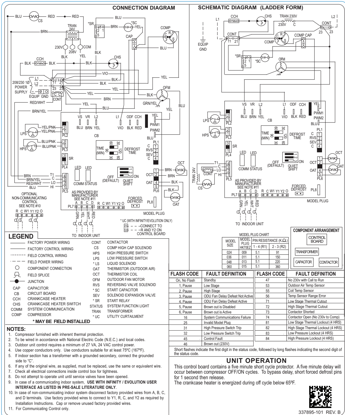
Fig. 1 – Wiring Diagram — Model size 3 tons, 208/230-1
